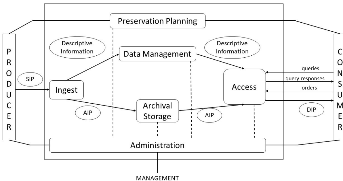
Fig. 2.1: OAIS Functional Entities
